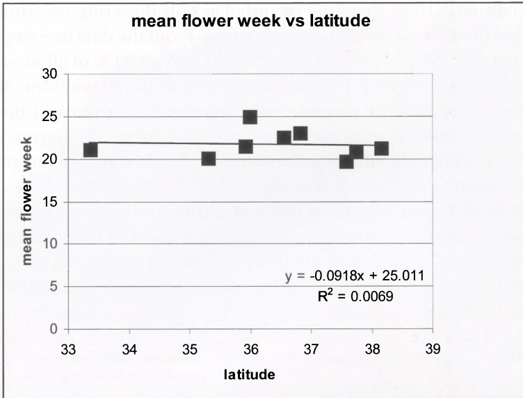
Figure 26. Mean flowering week versus latitude of the collection site in Korea for plants from the 1976 NAU expedition. Each data point represents all mean flowering week for the years 2004 through 2006 for all the accessions at a given site. First the mean of each accession was calculated and then the mean of these means was made to get these data.
