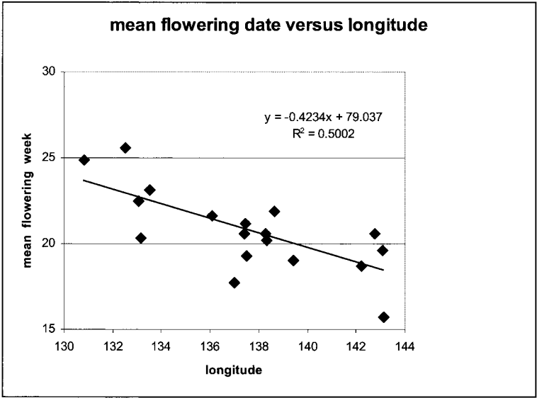
Figure 14. Mean week of flowering of plants from different collection areas in Japan versus longitude.
