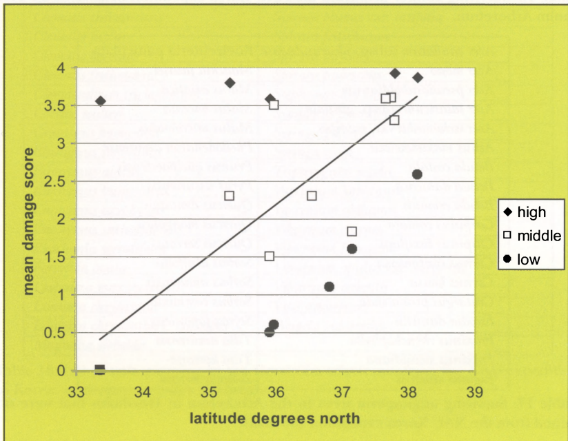
Figure 24. Summary of winter damage in Norway of material from the NAU 1976 expedition to Korea. The data is from table 13 in Sanda (1982). A damage score of zero was used to indicate dead plants while a score of 4 indicates no visible damage. Three elevation zones, high (1500-1749 m), middle elevation (750-999 m) and low (0-250 m). The regression line is fitted to the data from the middle elevation zone (score = 0.675 \cdot \text{latitude} - 22.12 , R^2 = 0.65 ).
