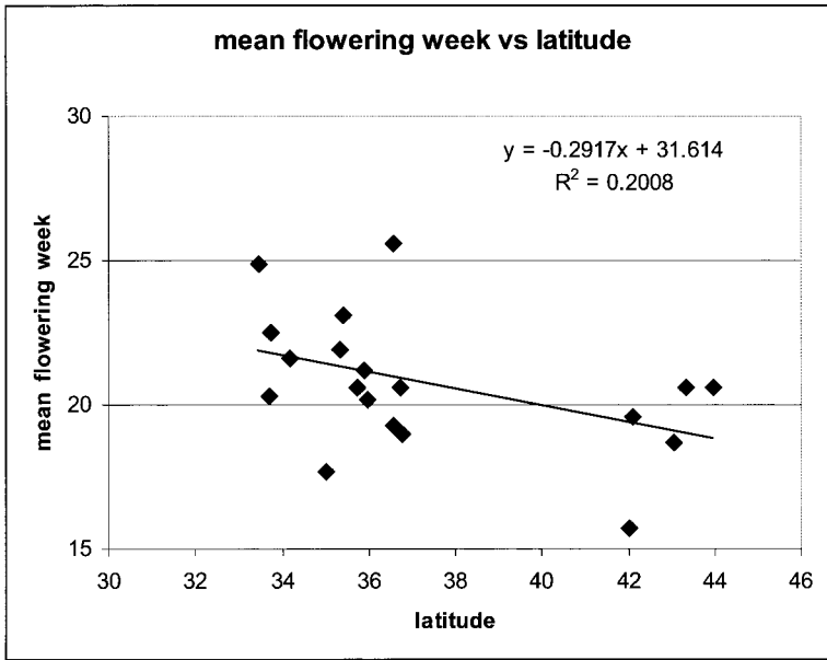
Figure 13. Mean flowering week versus latitude of the collection site in Japan for plants from the 1976 NAU expedition. Each data point represents all mean flowering week for the years 2004 through 2006 for all the accessions at a given site. First the mean of each accession was calculated and then the mean of these means was made to get these data.
