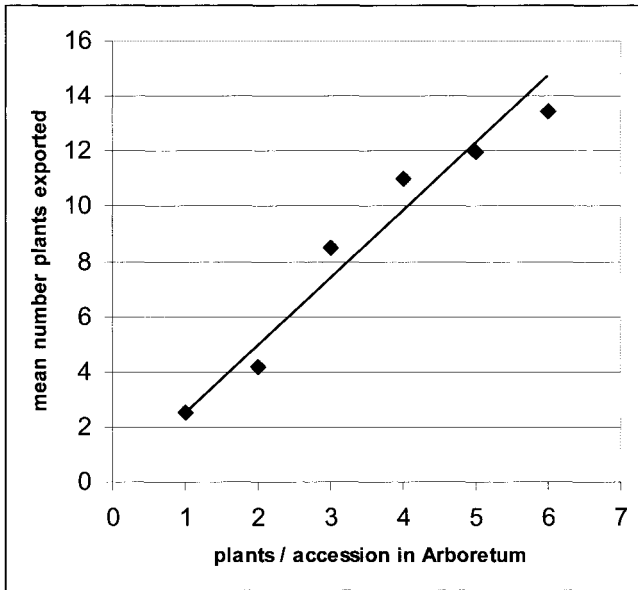
Figure 10. The average number of plants exported per accession plotted against the number planted out in the Arboretum when the number was less than 7. The regression line in the figure was forced through zero.
