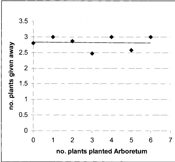
Figure 22. The average number of plants from the NAU expedition to Korea given away per accession versus the number planted out in the Arboretum in Hørsholm. The line represents a fitted linear regression ( R^2 = 0.002 ).
