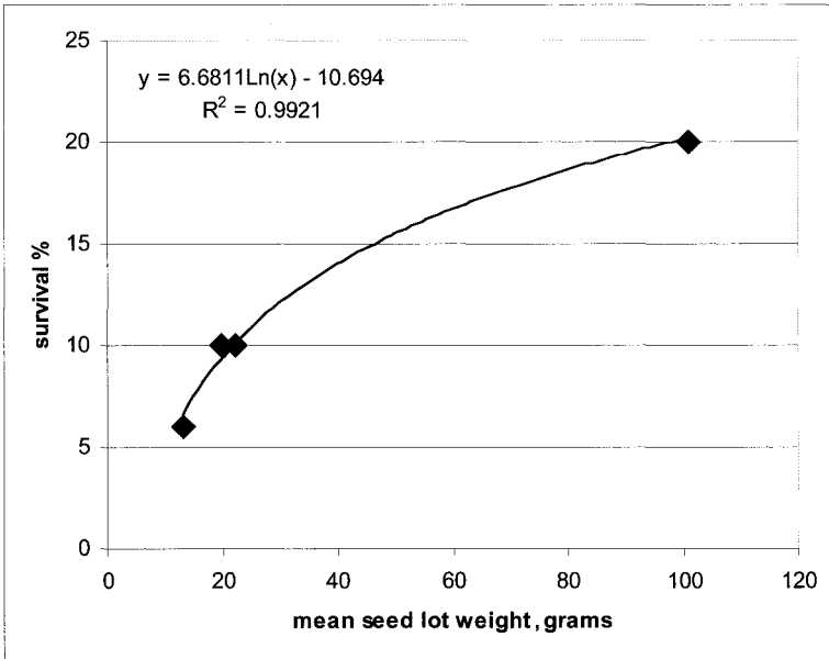
Figure 7. Mean survival of seed lots from different sources plotted against mean weight of seed in the seed lots.
